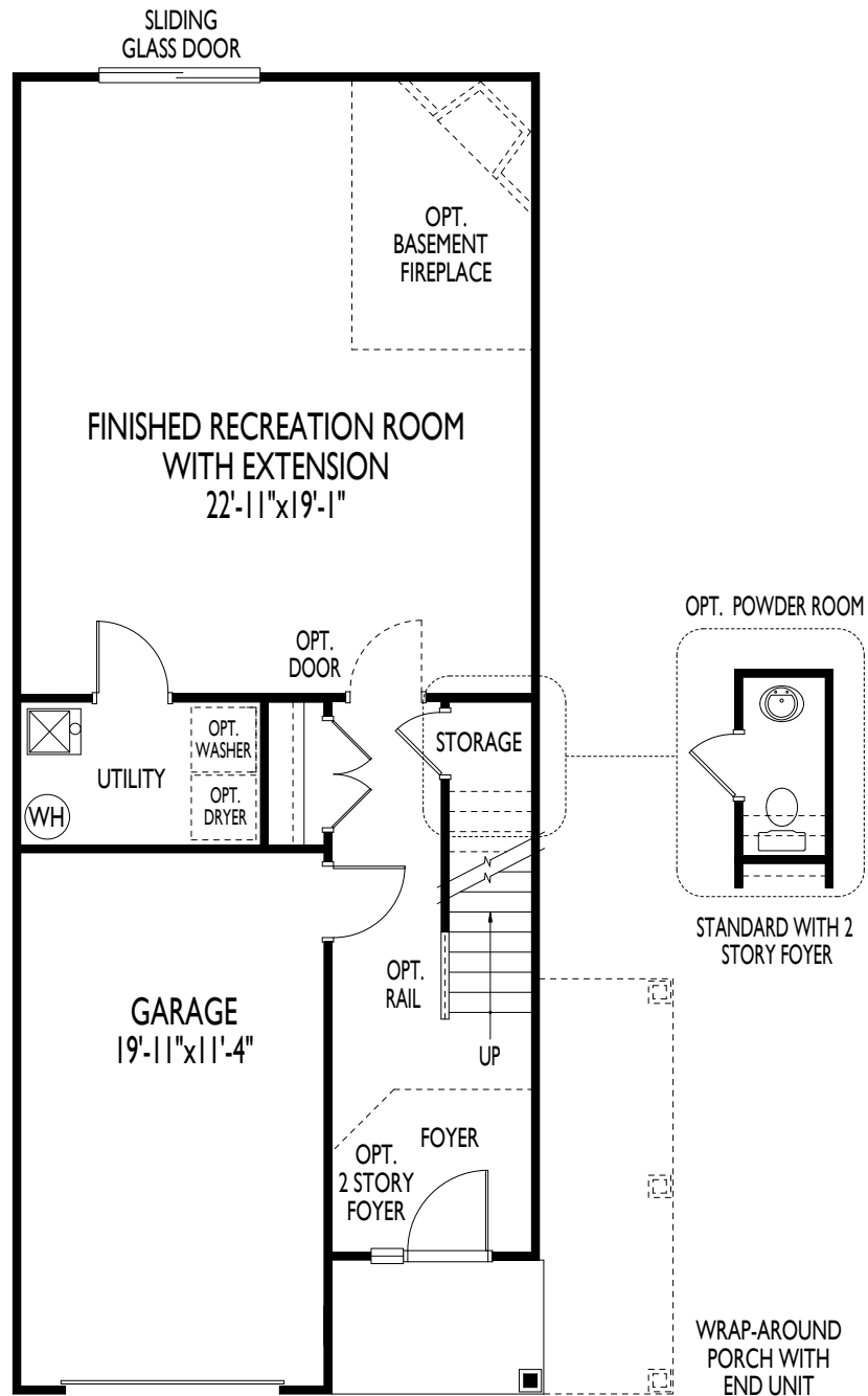
GROUND FLOOR WITH OPT. REAR 10' EXTENSION WITH OPTIONAL OVERLOOK AND FINISHED RECREATION ROOM
