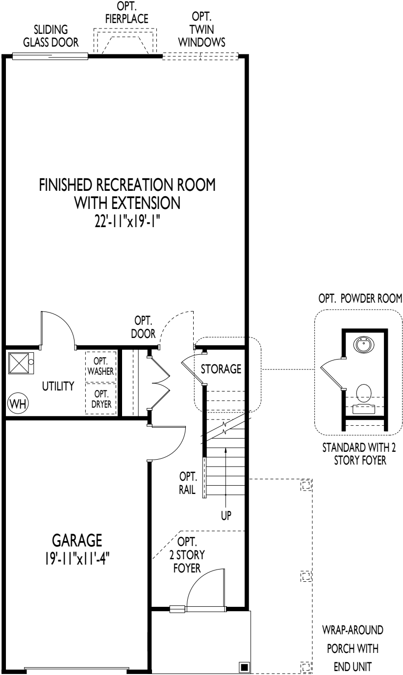
GROUND FLOOR WITH OPT. REAR 10' EXTENSION WITH FINISHED RECREATION ROOM
