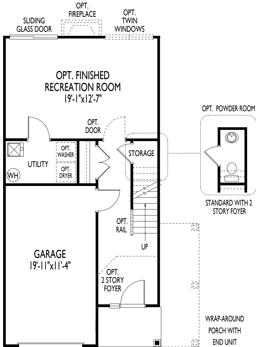
STANDARD GROUND FLOOR
