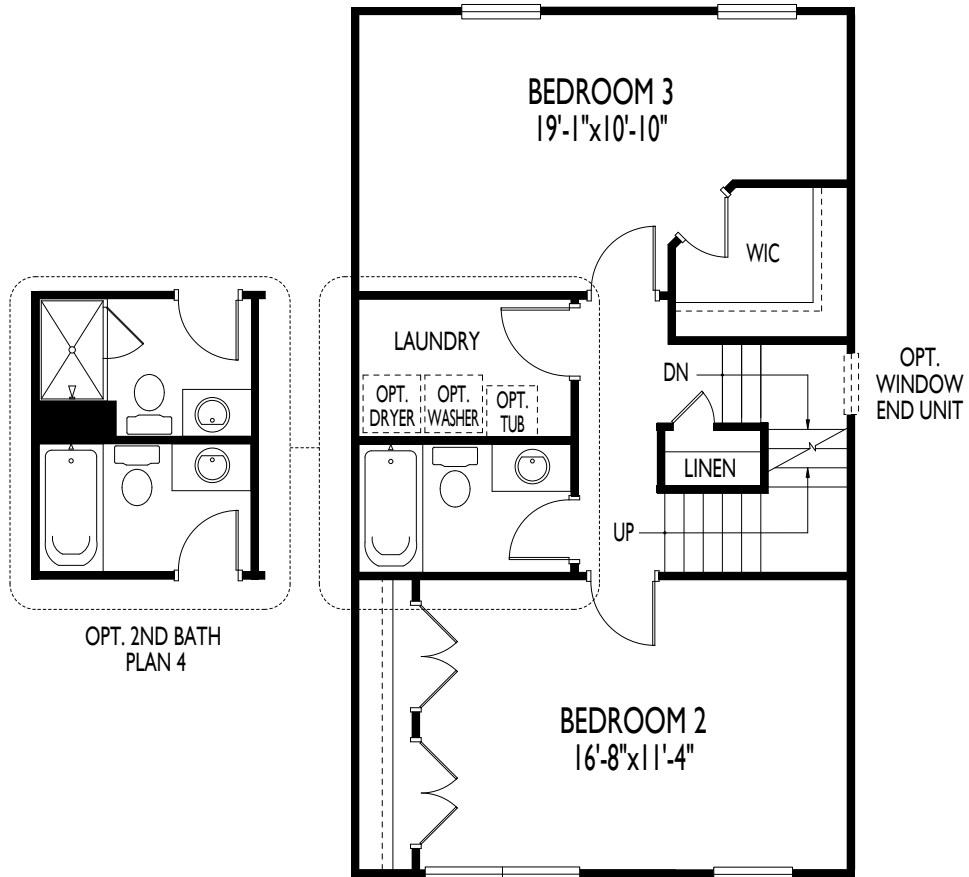
THIRD FLOOR WITH OWNERS' SUITE
