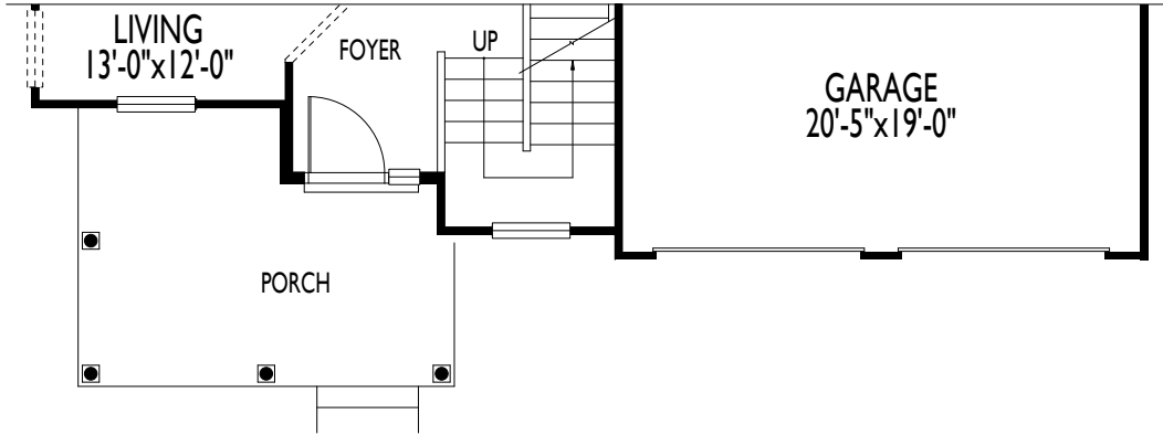
FIRST FLOOR PLAN - ELEV. 4
