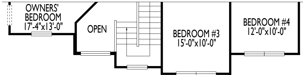
SECOND FLOOR PLAN - ELEV. 4
