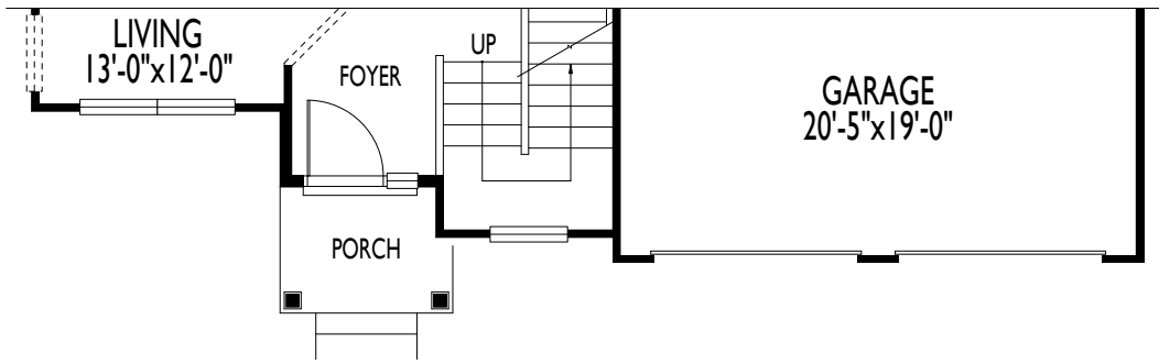
FIRST FLOOR PLAN - ELEV. 2
