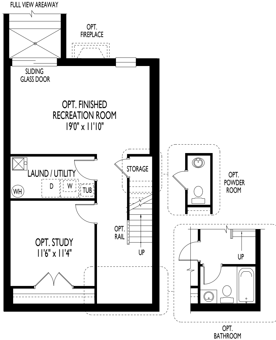
UNFINISHED RECREATION ROOM STANDARD GROUND FLOOR - PLAN 1 FINISHED RECREATION ROOM - PLAN 2
