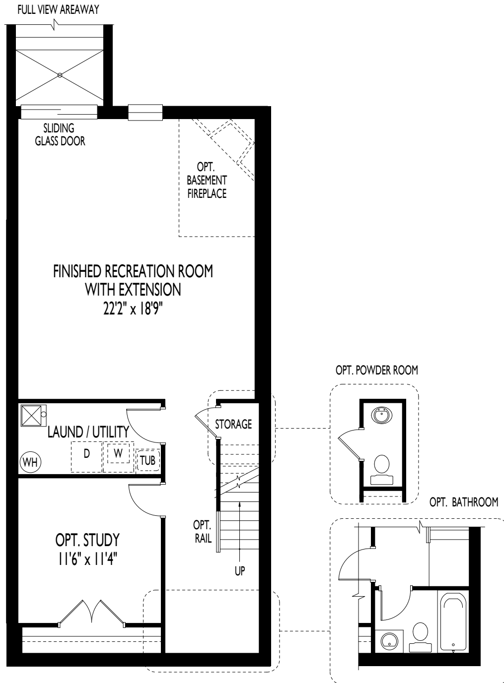
GROUND FLOOR WITH FINISHED RECREATION ROOM WITH OPT. REAR 10' EXT. OVERLOOK - PLAN 4
