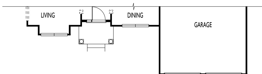
PARTIAL FIRST FLOOR PLAN - ELEVATION 3
