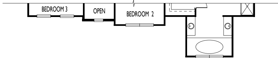
PARTIAL SECOND FLOOR PLAN - ELEVEATION 4
