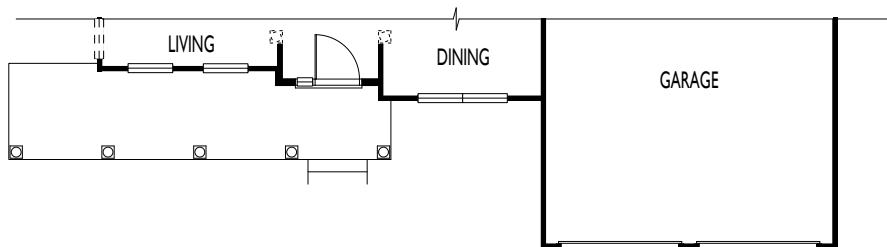
PARTIAL FIRST FLOOR PLAN - ELEVATION 4
