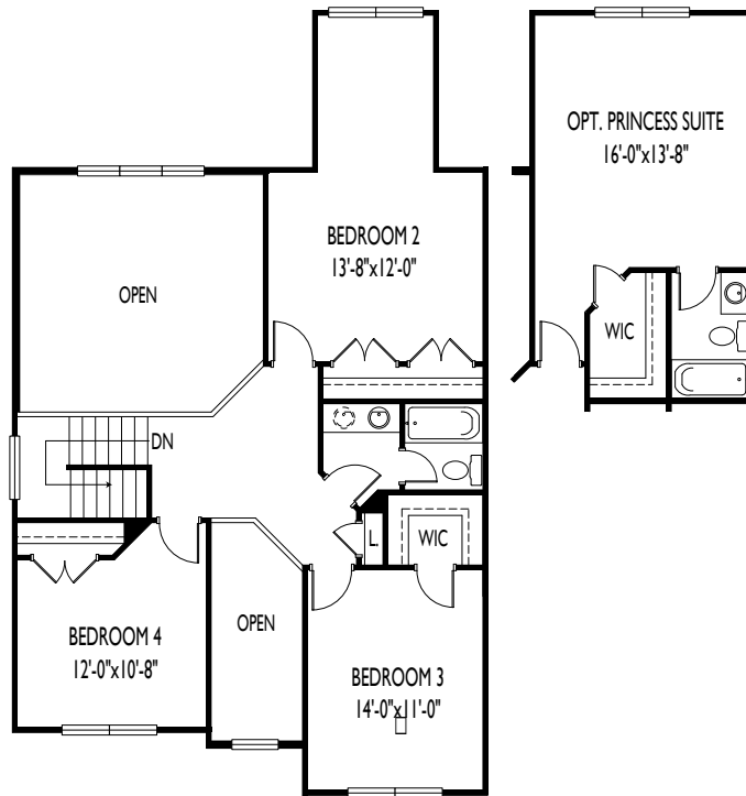
SECOND FLOOR PLAN - ELEVATION 1
