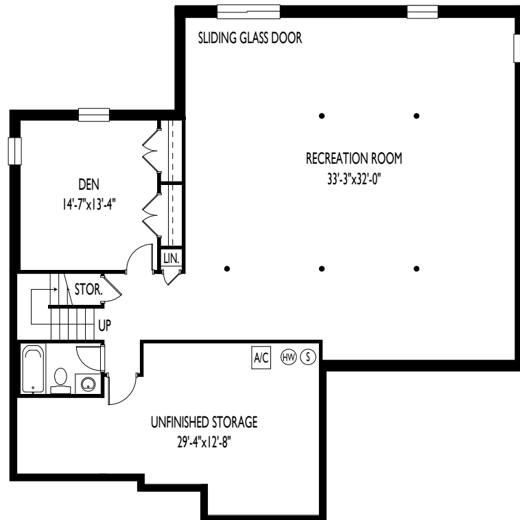
THE DELANEY- FINISHED BASEMENT FLOOR PLAN
