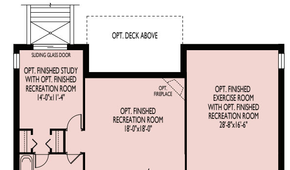
OPT. FINISHED BASEMENT PLAN WITH OPT. AREAWAY
