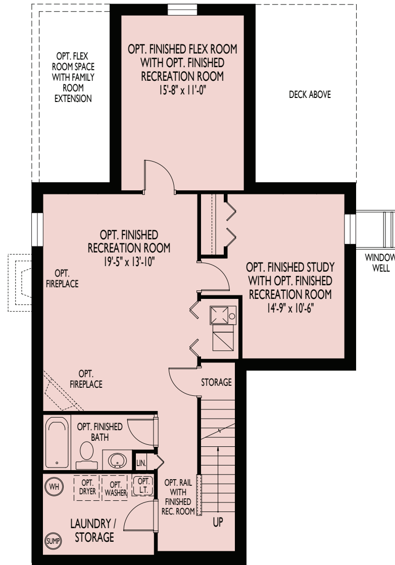
OPT. FINISHED BASEMENT FLOOR PLAN
