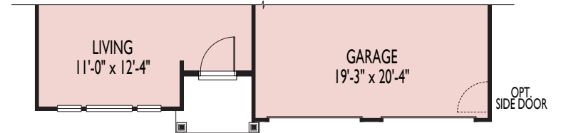
PARTIAL FIRST FLOOR PLAN - ELEVATION 2
