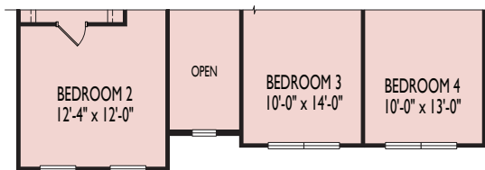
PARTIAL SECOND FLOOR PLAN - ELEVATION 3
