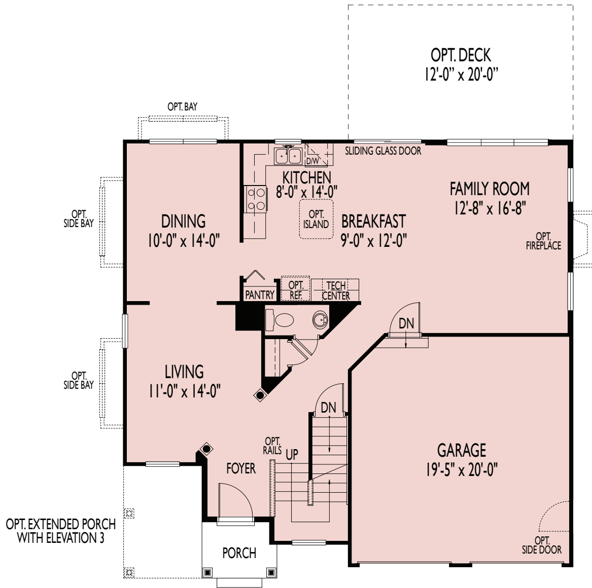
FIRST FLOOR PLAN - ELEVATION I
