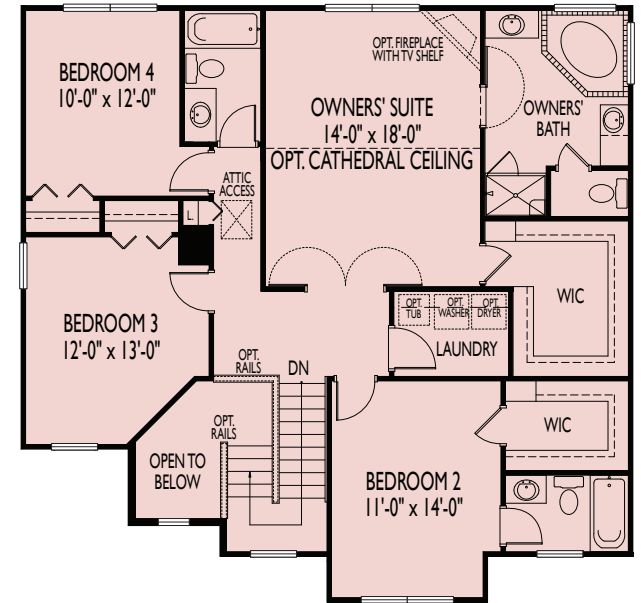
OPTIONAL SECOND FLOOR PLAN 2
