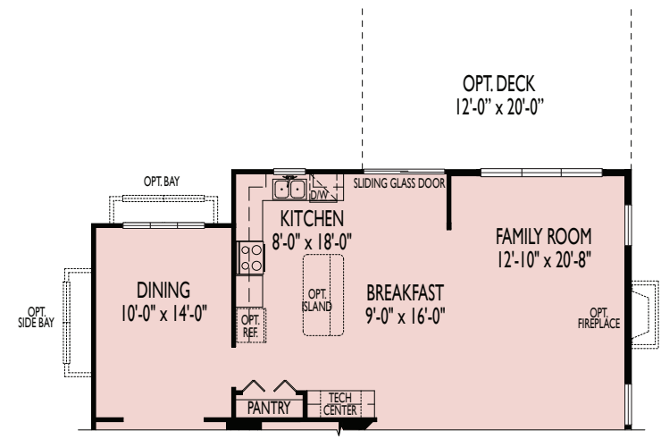
FIRST FLOOR PLAN WITH OPT. 4' KITCHEN / BREAKFAST / FAMILY ROOM EXTENSION
