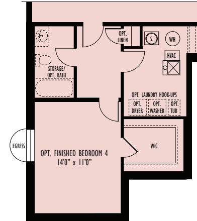
OPT. FINISHED 4TH BEDROOM PLAN (AVAILABLE WITH OPT. FINISHED RECREATION ROOM ONLY)
