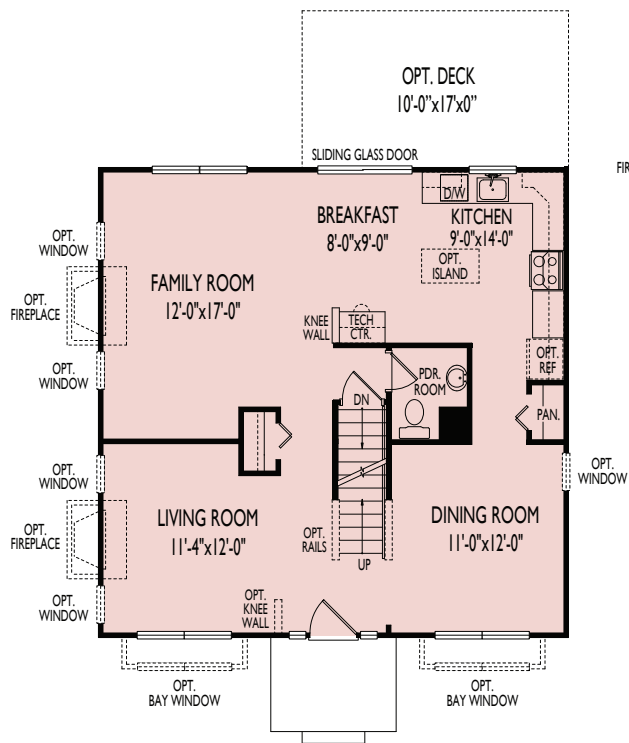
FIRST FLOOR - ELEVATION I
