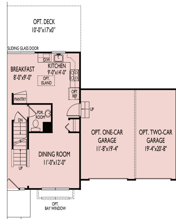
FIRST FLOOR - ELEVATION I - WITH OPT. ONE AND TWO-CAR GARAGE
