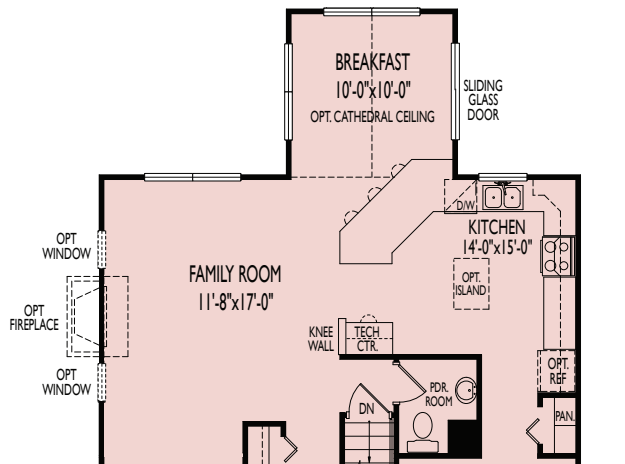
FIRST FLOOR PLAN - WITH OPT. BREAKFAST AREA EXTENSION
