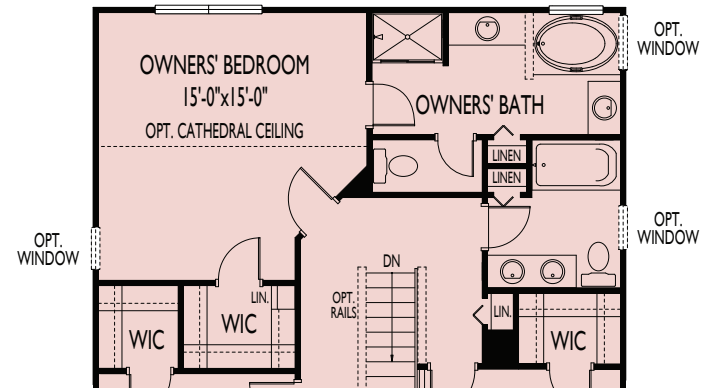
SECOND FLOOR - WITH OPT. THREE BEDROOM & 2' REAR EXTENSION
