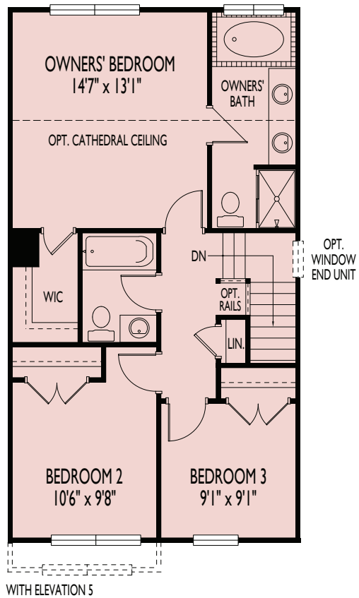
BEDROOM FLOOR PLAN WITH OPT. 2' EXTENSION
